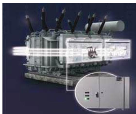
G9 Gas And Bushing PD, HEE & TFC - TOTUS (HV & MV)
