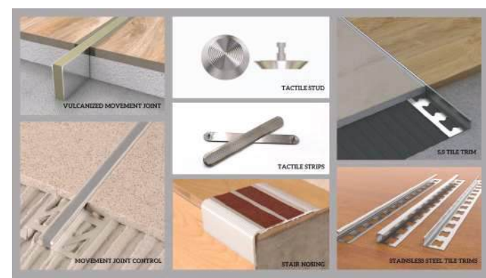
Finishing Profiles
