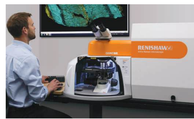
Raman Spectroscopy
